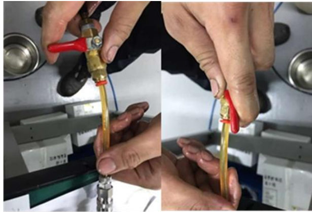
Figure 19 - Oil Filled-4
