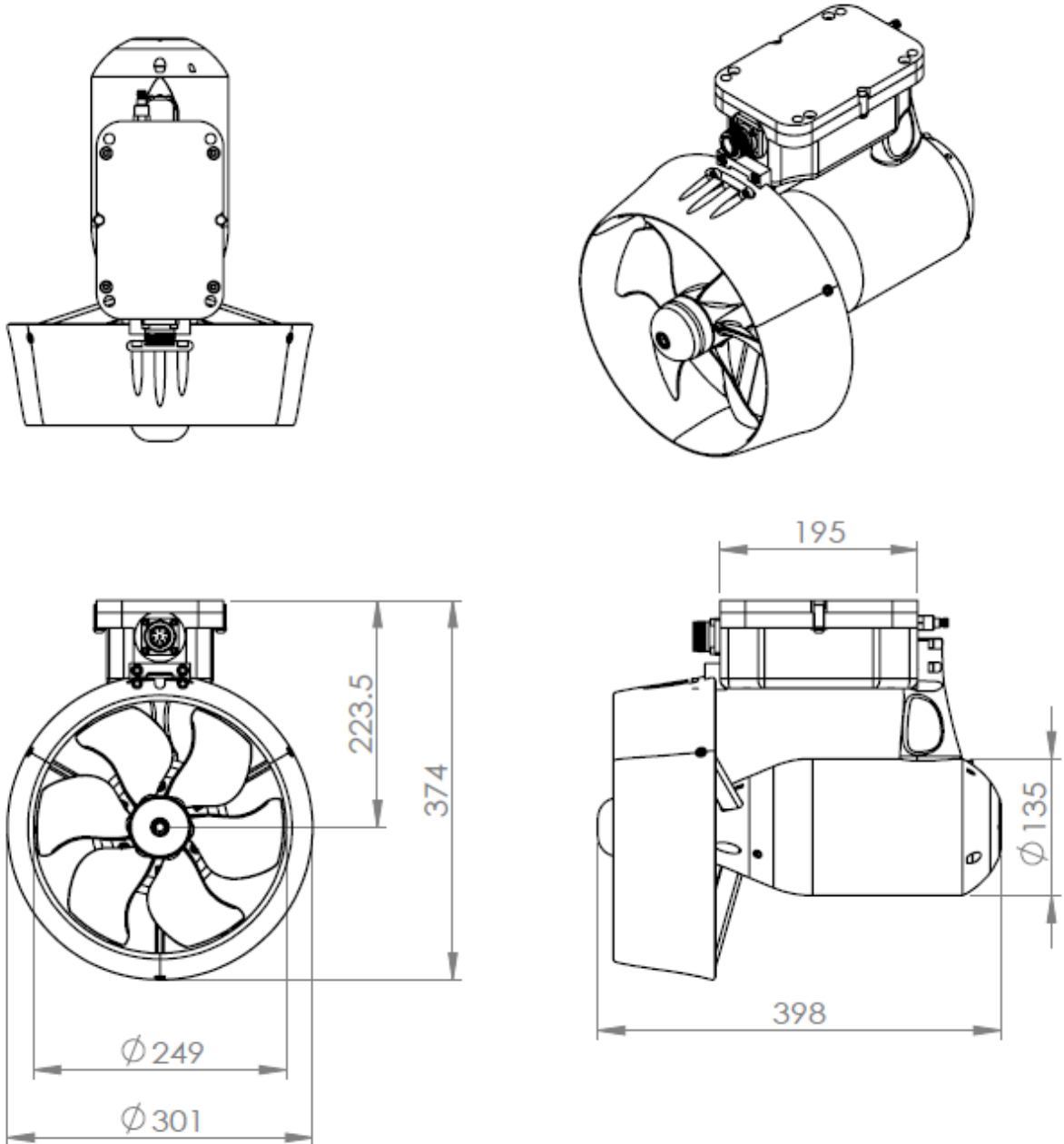
Figure 1 - DWT135D4 Thruster
