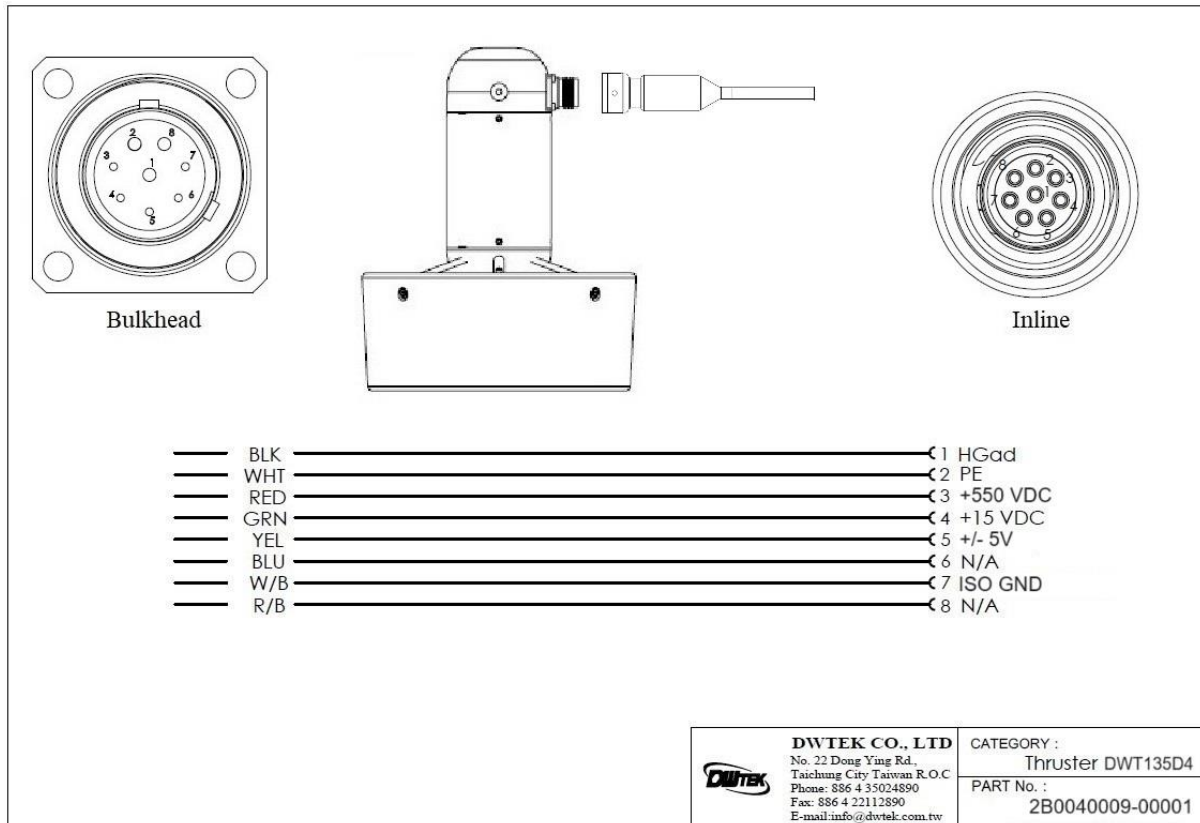
Figure 3 - DWT135D4 Thruster Pin Assignment
