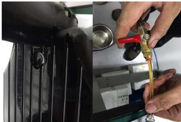
Figure 20 - Oil Filled-5
