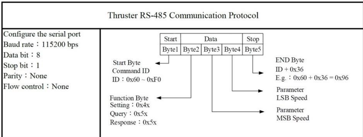
Figure 32 - Thruster RS-485 Communication Protocol
