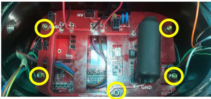
Figure 12 - Control Board Installation-9
