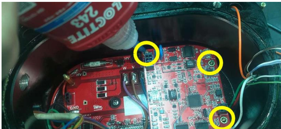
Figure 9 - Control Board Installation-6
