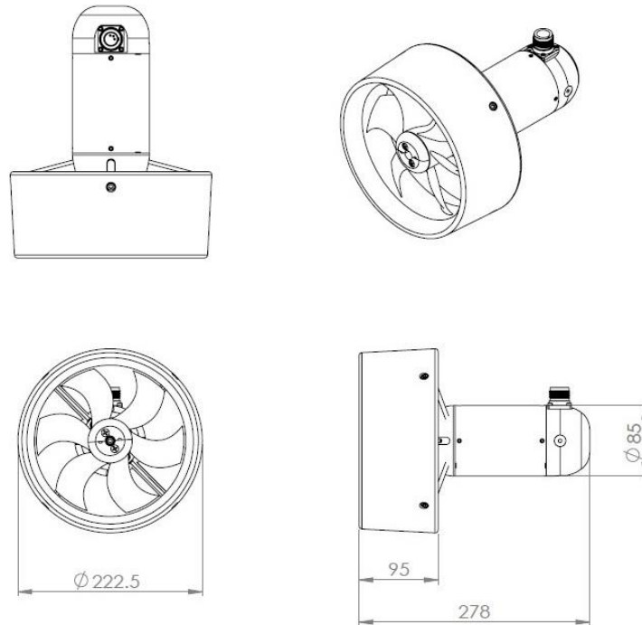
Figure 1 - DWT085G1 Thruster
